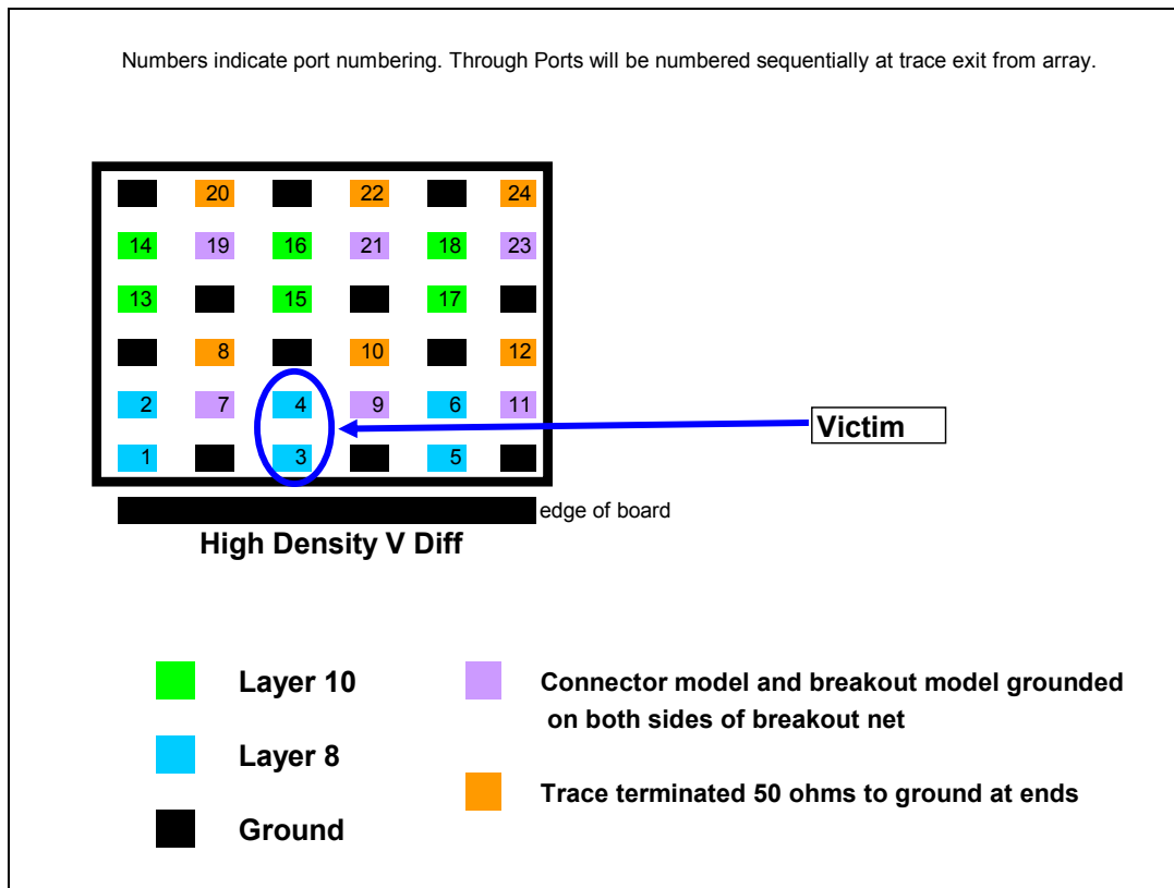
Figure 2 – RapidIO XMC connector to Final Inch Test Board Mapping
