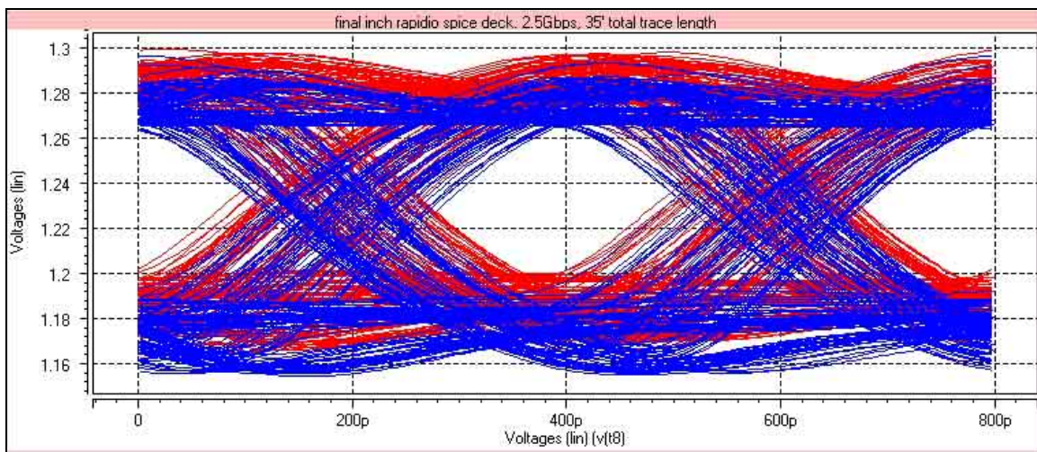
Picture 2 – RapidIO circuit eye waveform at 2.5 Gbps, probed at terminator pins, 35 inches total trace length
