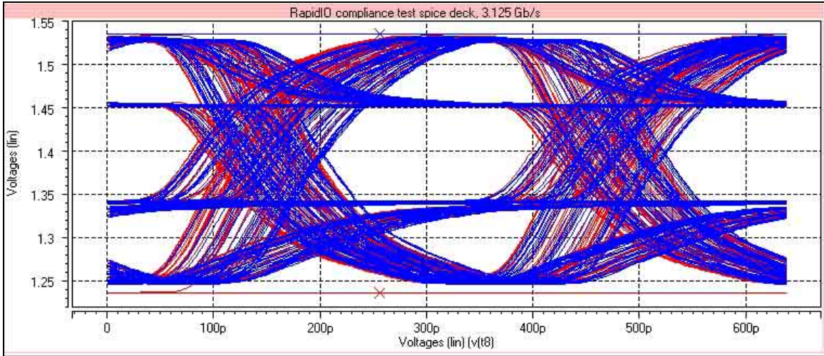
Picture 3 – Worst case stimulus eye waveform at 3.125 Gbps, probed at Xilinx driver package pins, connected to compliance test/measurement load
