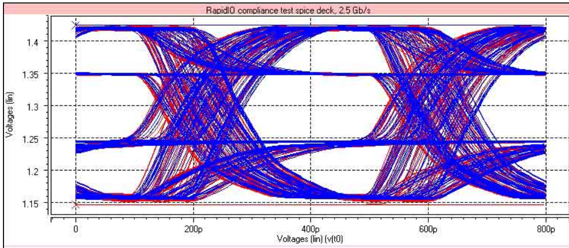
Picture 1 – Worst case stimulus eye waveform at 2.5 Gbps, probed at Xilinx driver package pins, connected to compliance test/measurement load
