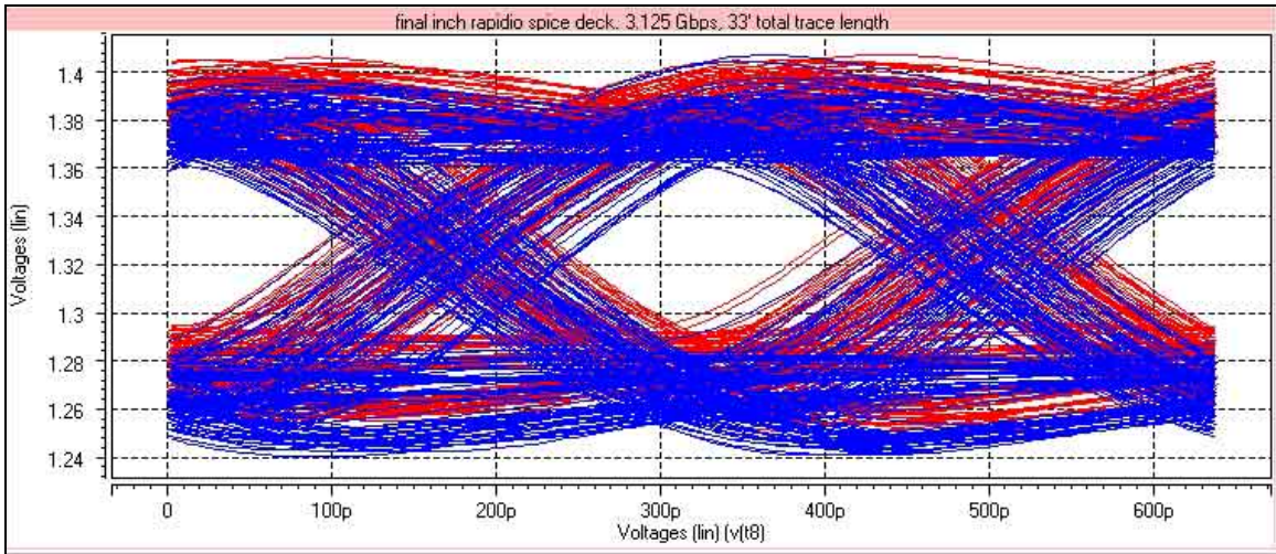
Picture 4 – RapidIO circuit eye waveform at 3.125 Gbps, probed at terminator pins, 33 inches total trace length
