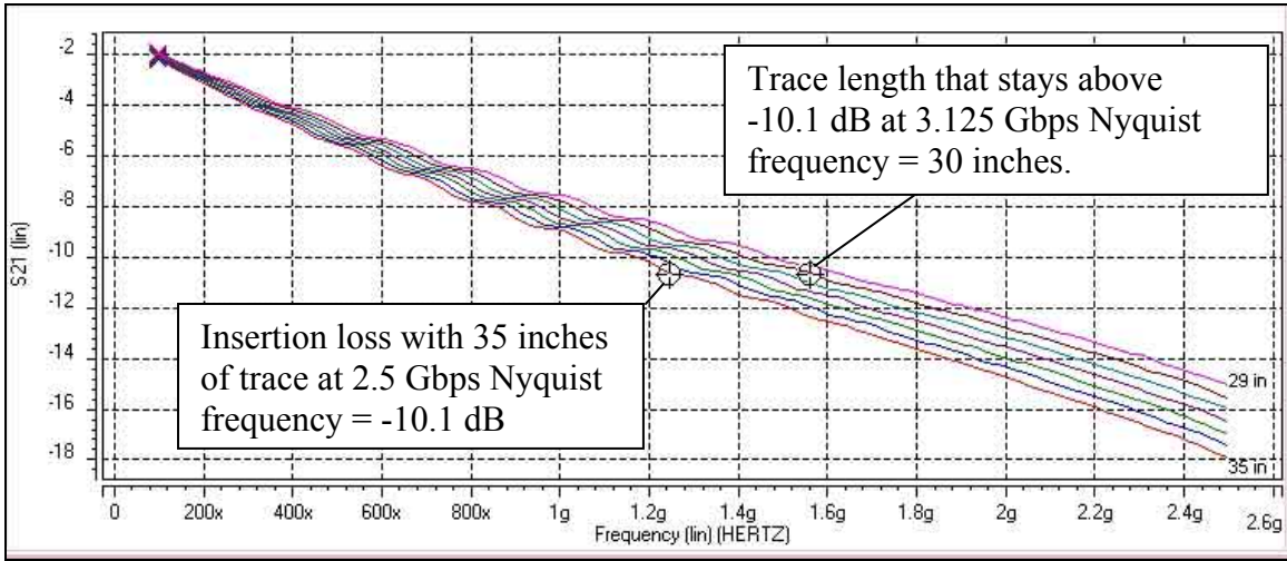
Figure 5 - RapidIO circuit insertion loss at trace lengths between 29 inches and 35 inches
