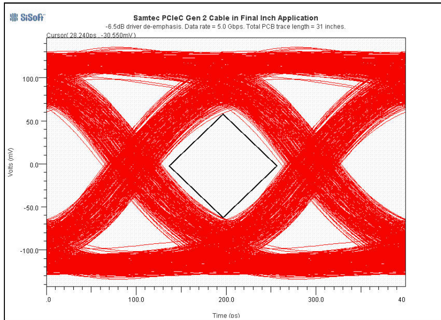
Picture 7 – Receiver eye measurement, probed at far end termination. Standard driver setting with -6.5 dB de-emphasis. Total trace length = 31 inches.
