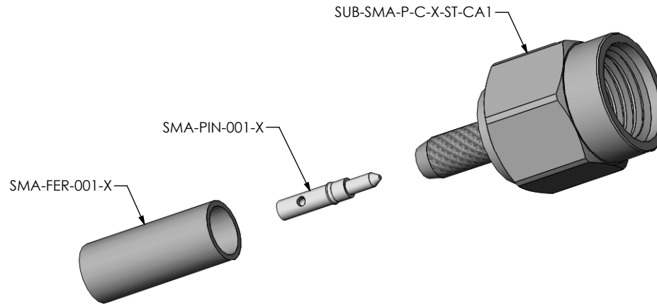
FIG.1 SMA-P-C-X-ST-CA1 SHOWN
